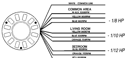
Wiring Diagram
